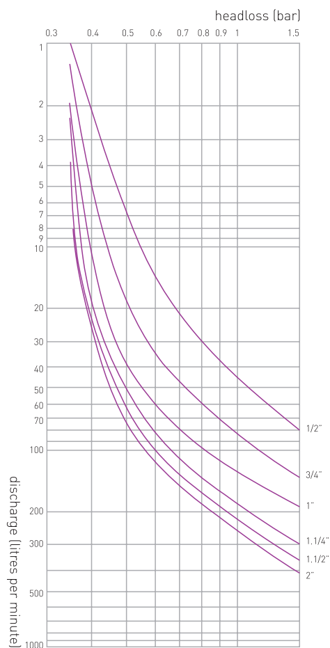
discharge and headloss diagram
